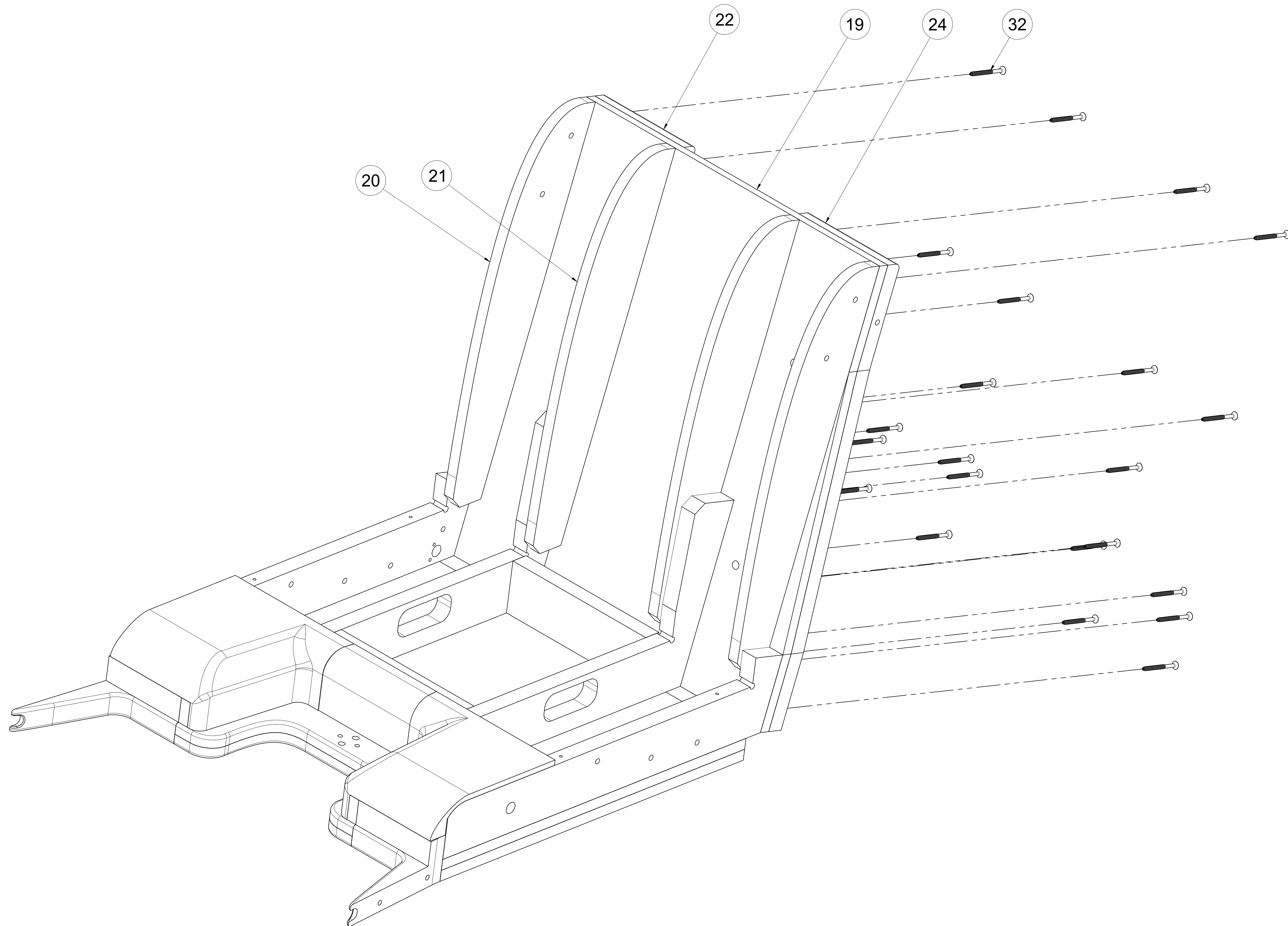
-1000 ASSY SEAT BACK ASSEMBLY
