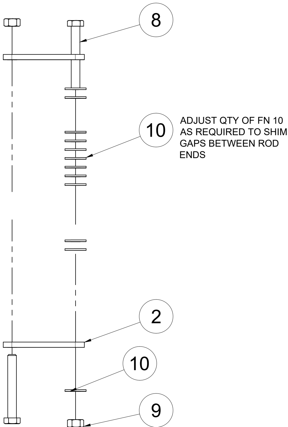
-1 ASSY PARACHUTE ROCKET LINK ASSEMBLY
