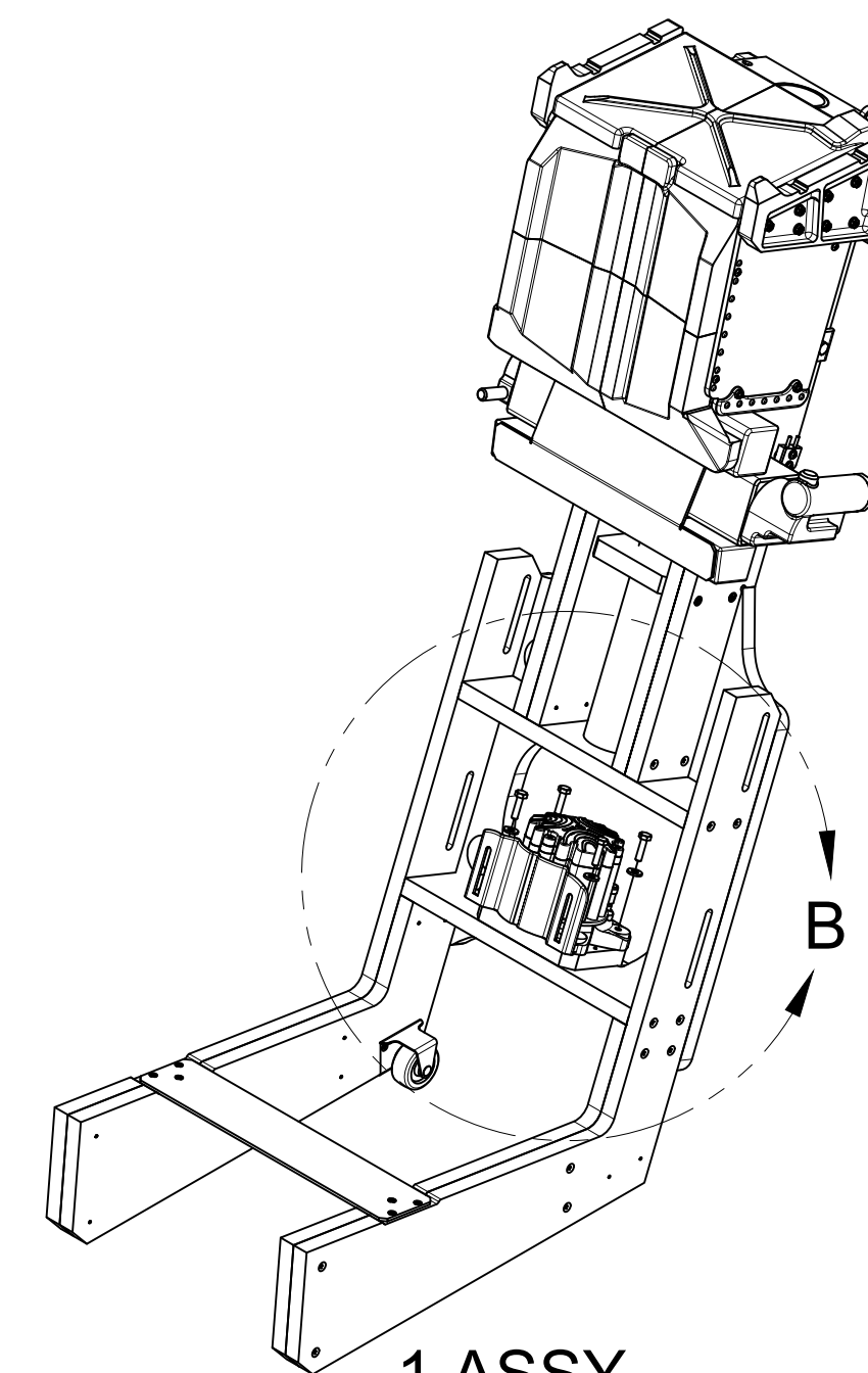
-1 ASSY TRANSDUCER (BUTTKICKER) INSTALLATION
