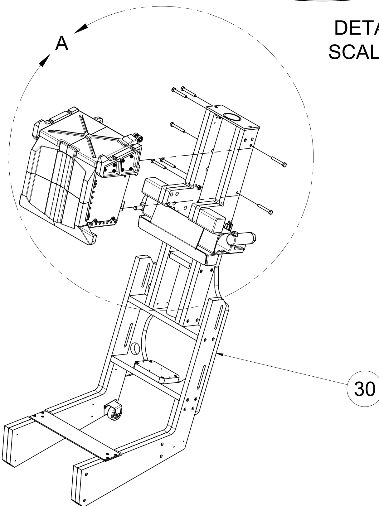
-1 ASSY PARACHUTE CONTAINER (HEADREST) INSTALLATION
